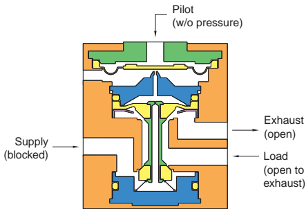
Valve Closed
